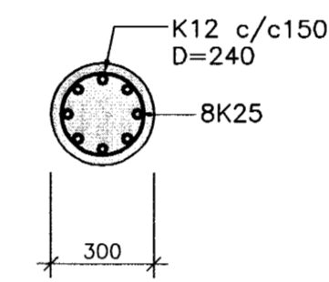
SNID E 1:20 B42
