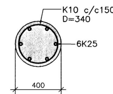
SNID C 1:20 B42
