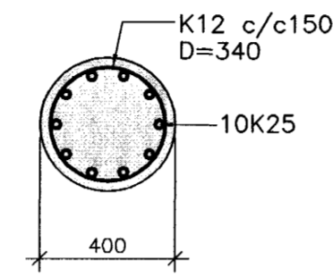
SNID A 1:20 B42
