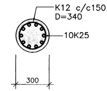
SNID D 1:20 B42
