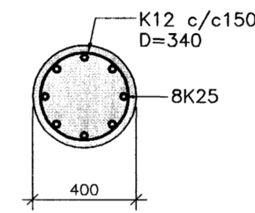
SNID B 1:20 B42
