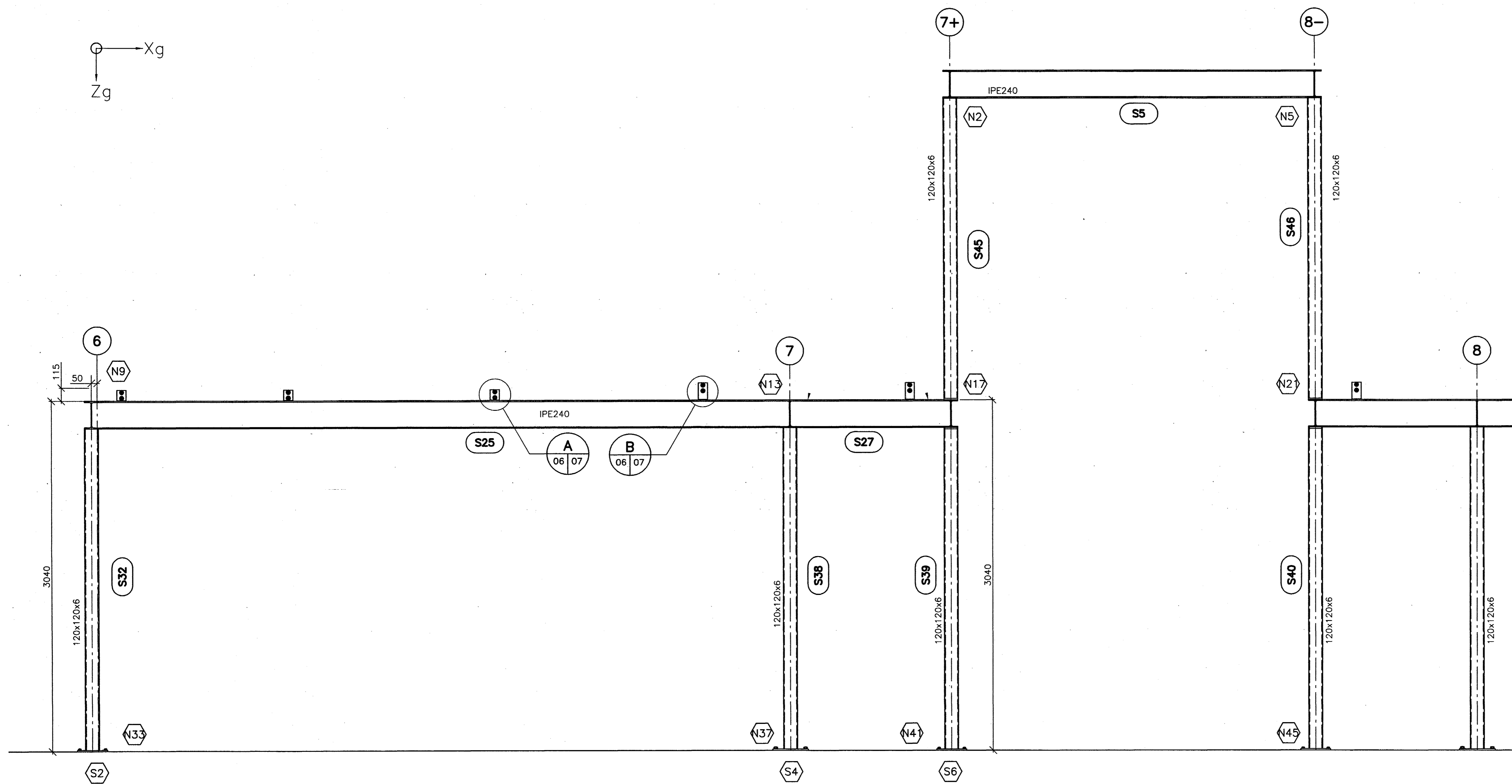
5 SECTION 02 | 06 SCALE 1:20
