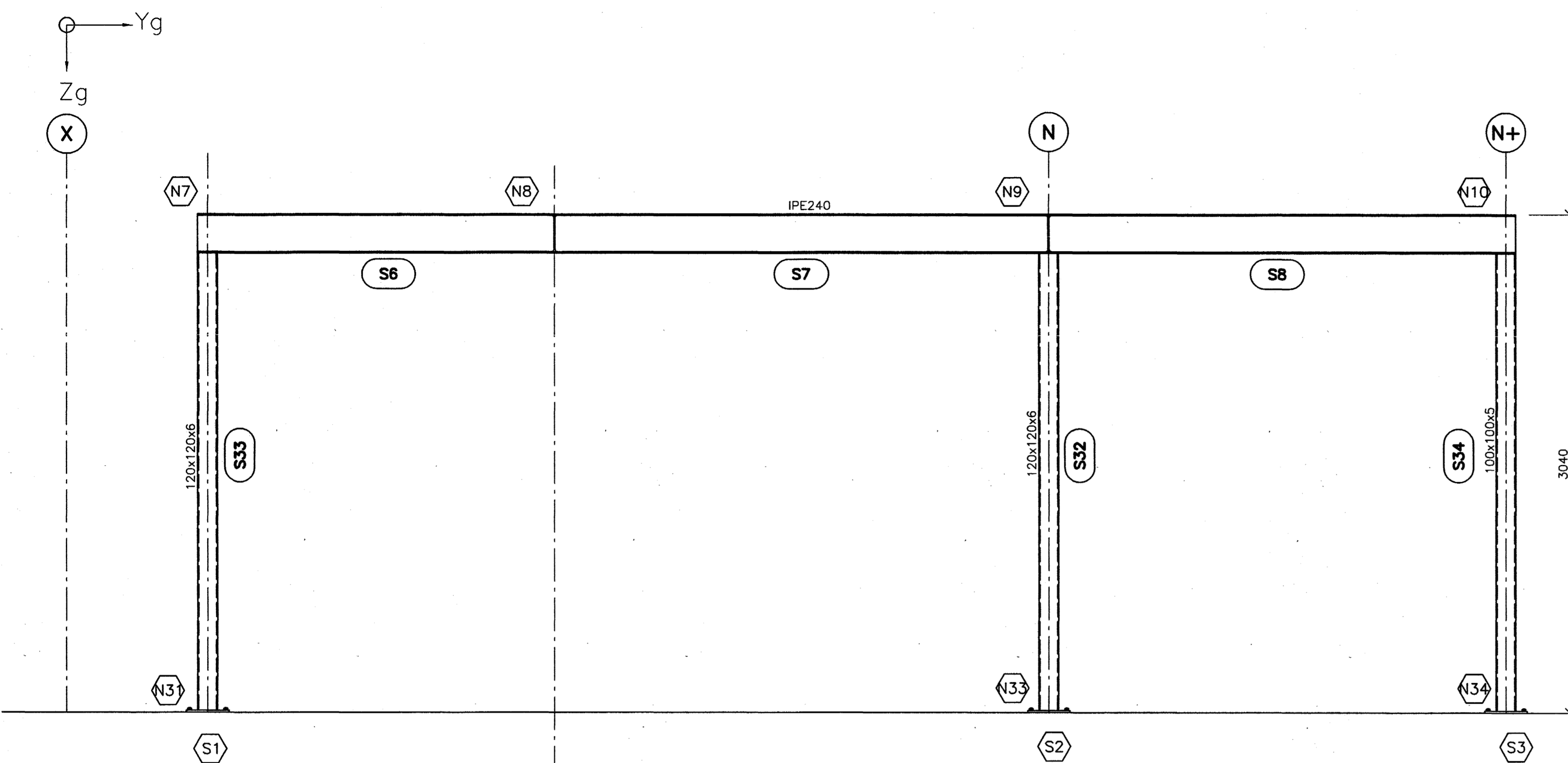
1 SECTION 02 03 SCALE 1:20
