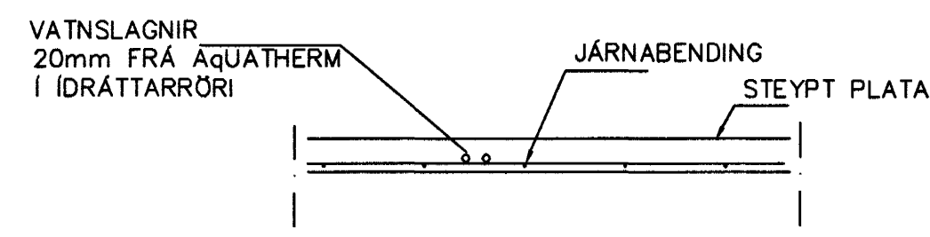
LAGNIR, SNID, 1:20
