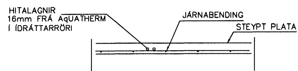
LAGNIR, SNID, 1:20
