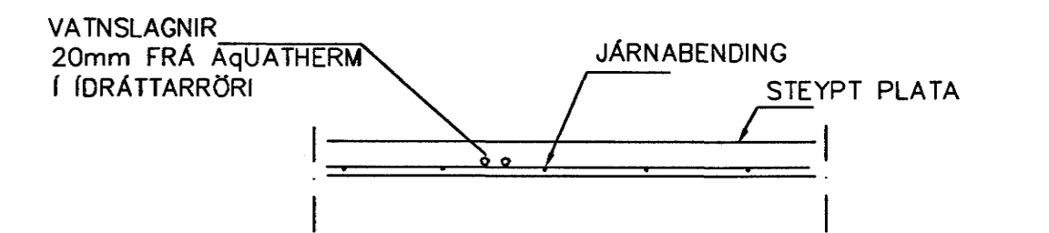
LAGNIR, SNID, 1:20
