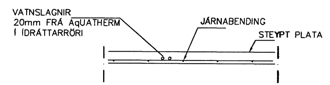
LAGNIR, SNID, 1:20
