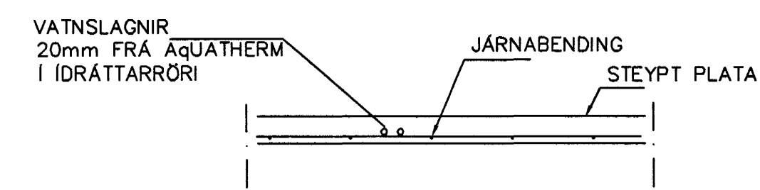
LAGNIR, SNID, 1:20
