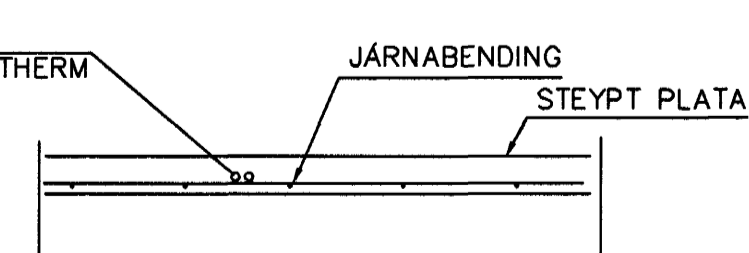
LAGNIR, SNID, 1:20
