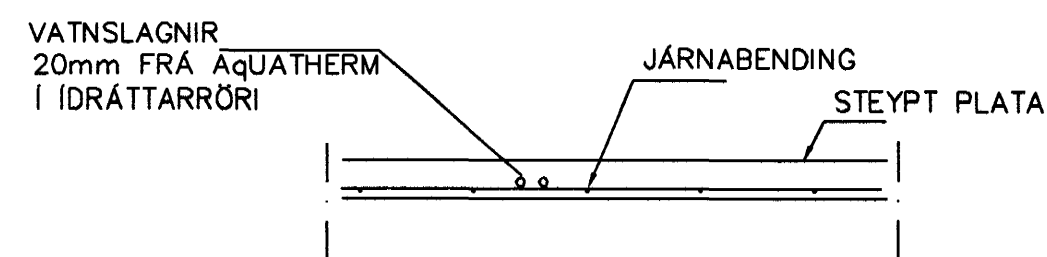
LAGNIR, SNID, 1:20
