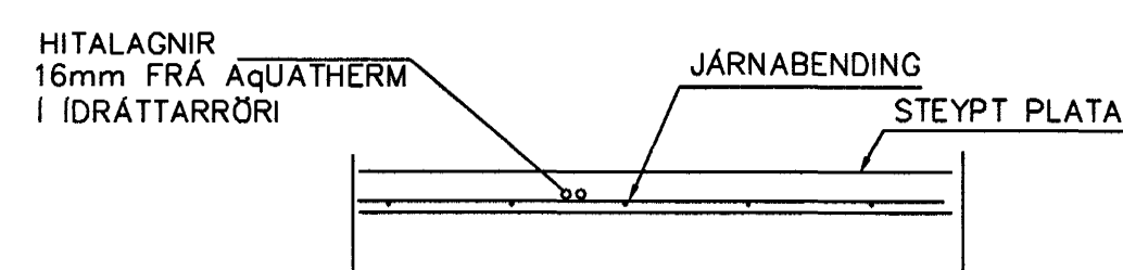
LAGNIR, SNID, 1:20
