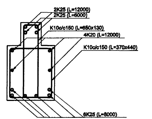
SNID C 1:20 C-B2 SV-07
