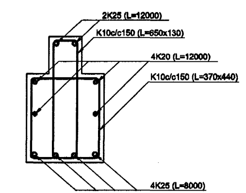
SNID D 1:20 C-B2 SV-07
