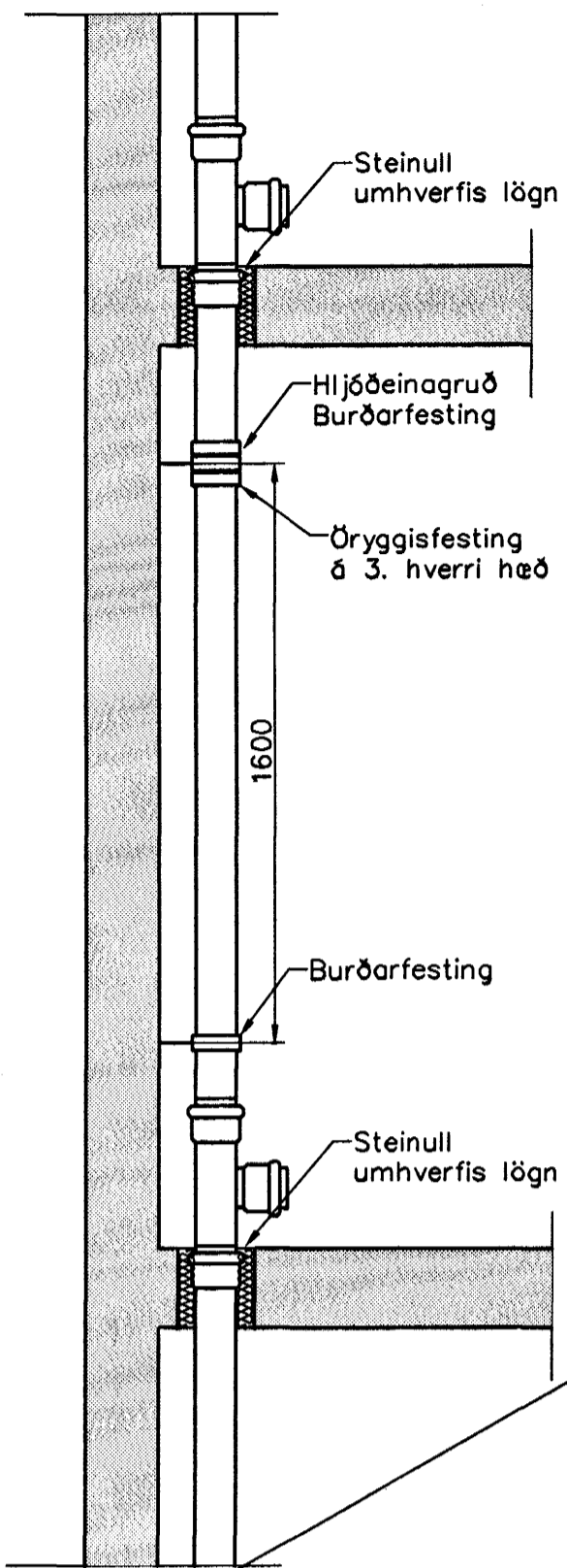
Fallpipa, festingar 1:20
