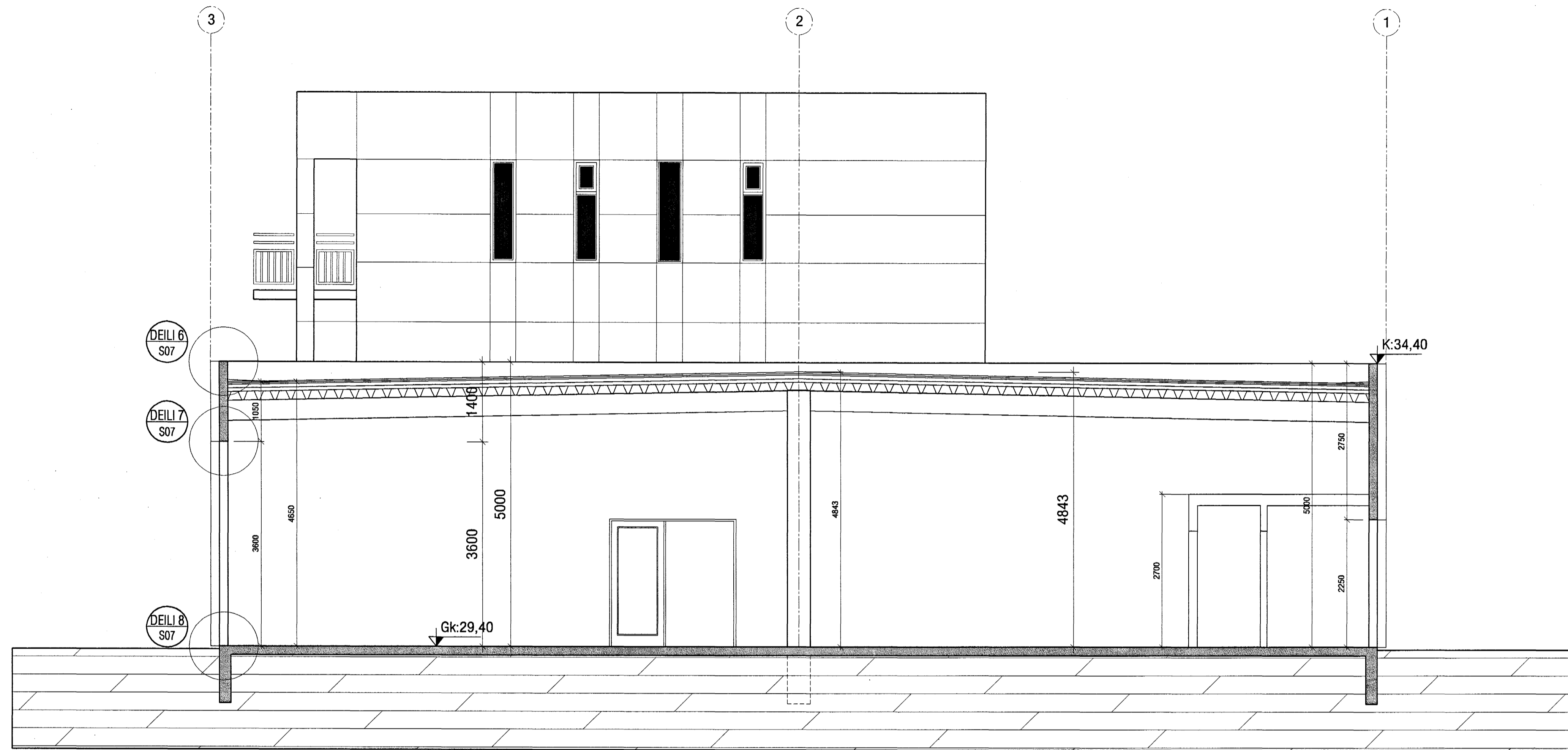
SNID B-B
