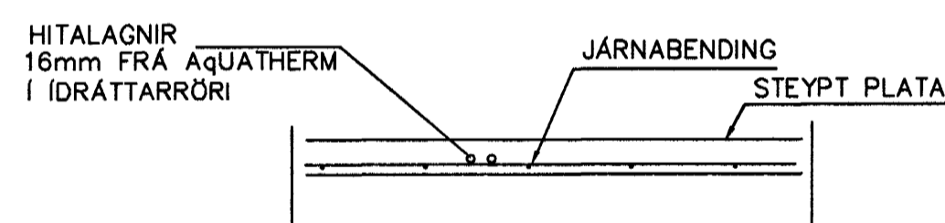
LAGNIR, SNID, 1:20
