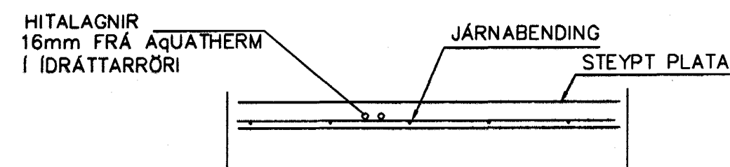
LAGNIR, SNID, 1:20
