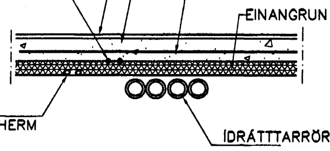
LAGNIR, SNID, 1:20
