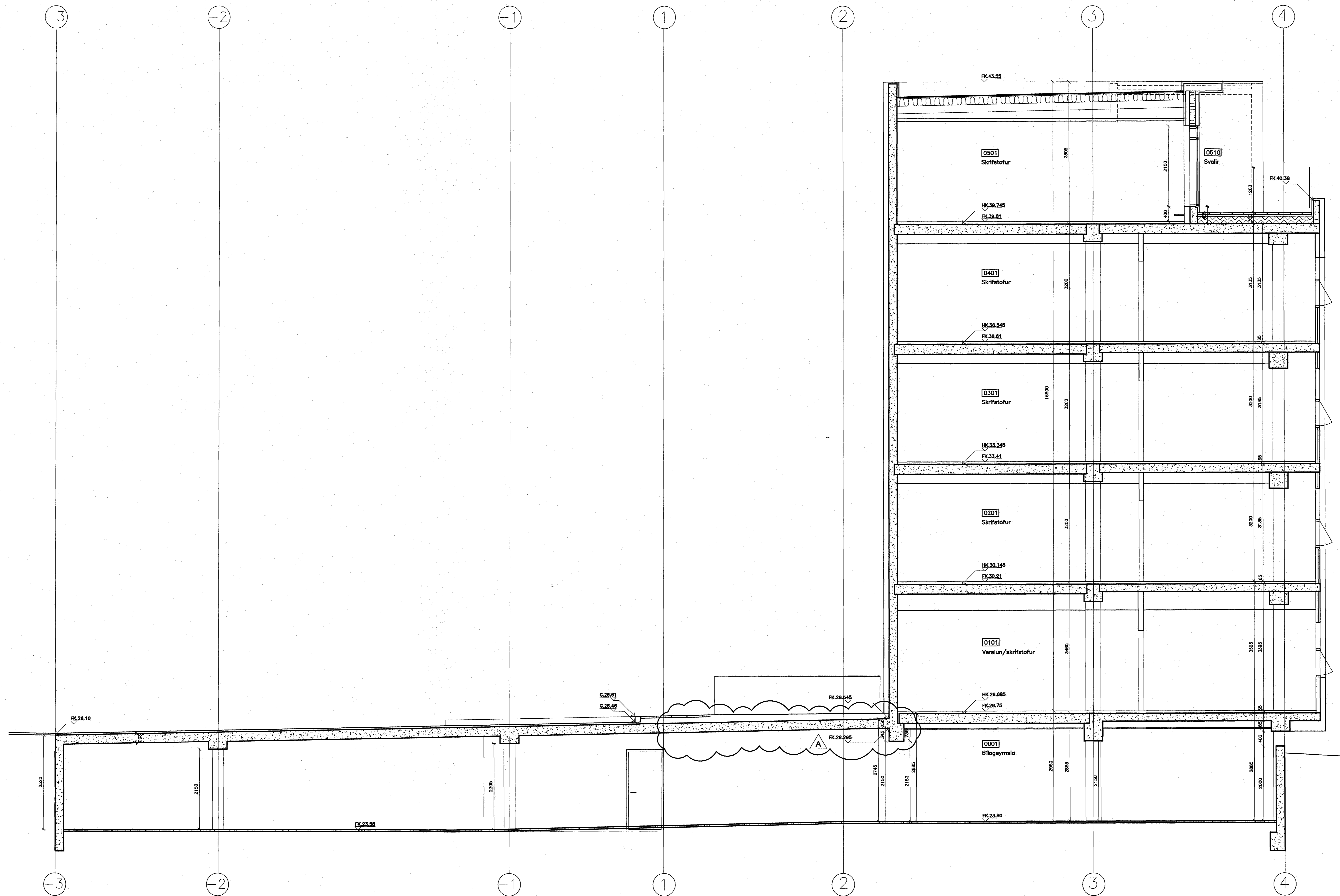
SNID G-G
