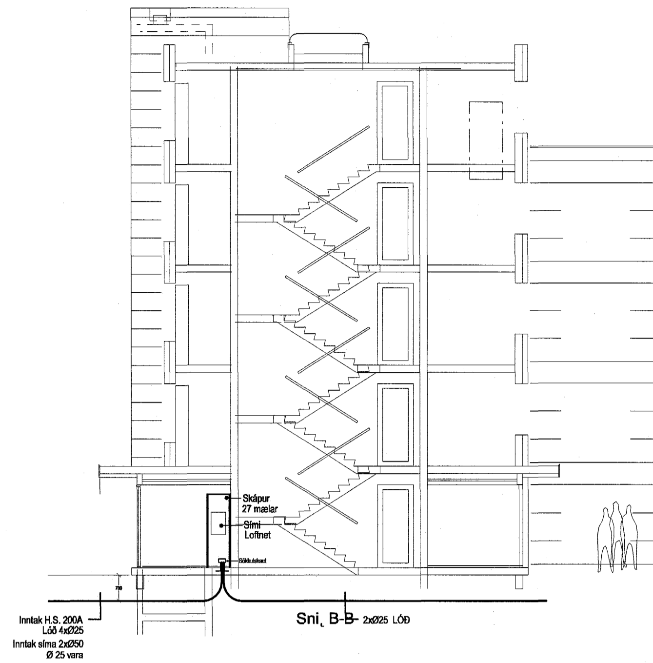
SNID, MKV. 1:100
