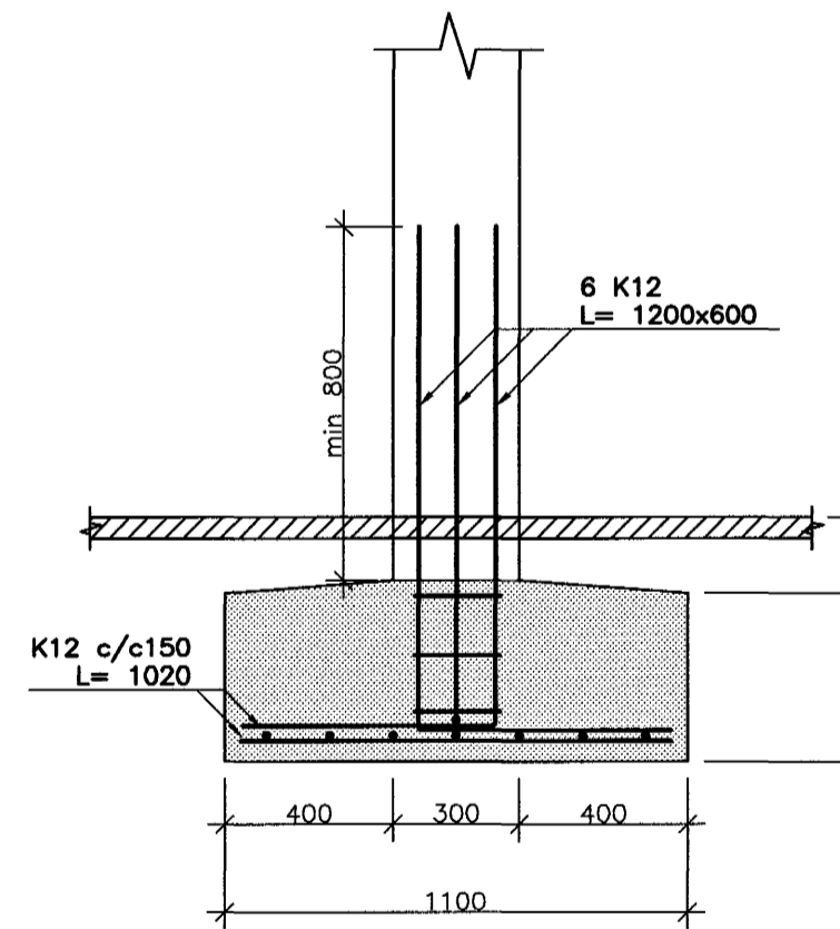
SNID B1 1:20
