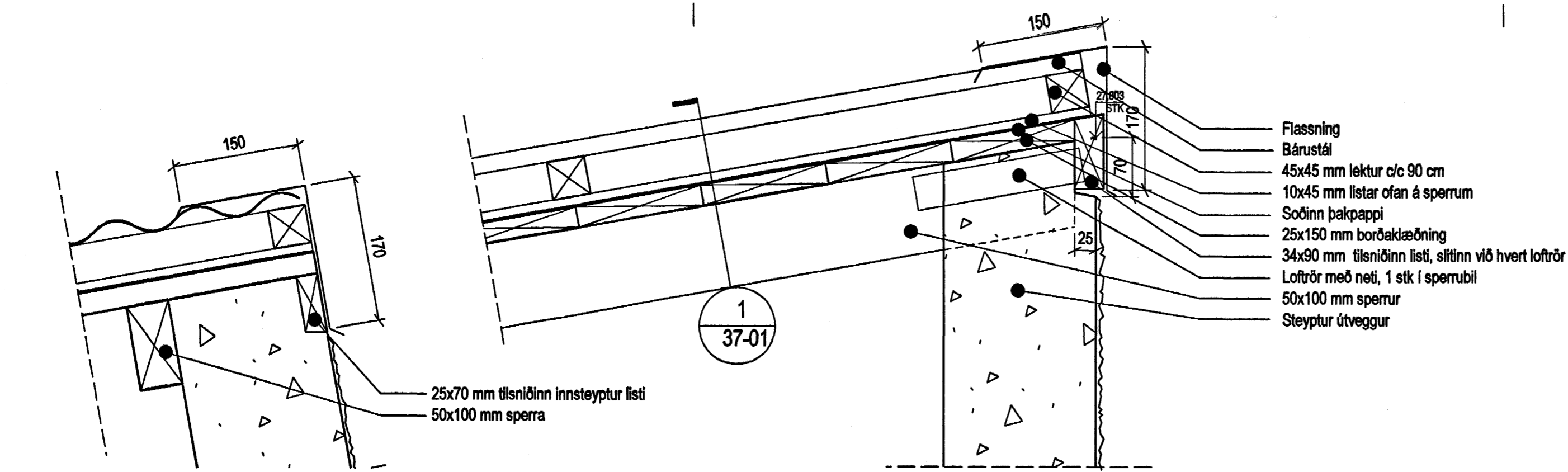
1 37-01 20-03 DEILI 1:5 Hallandi þak-gaflar
