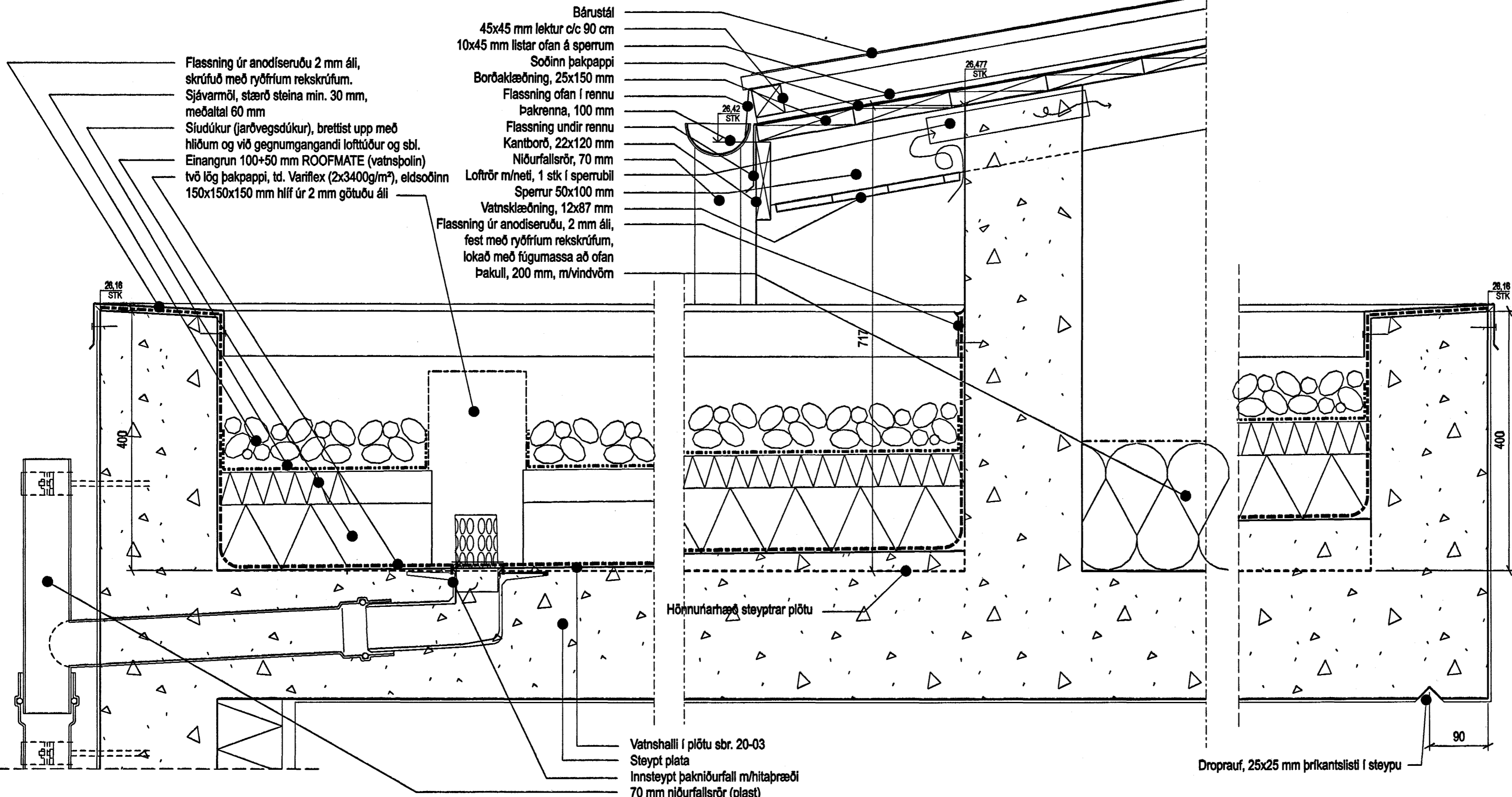
1 37-01 20-03 DEILI 1:5 Hallandi þak-gaflar
