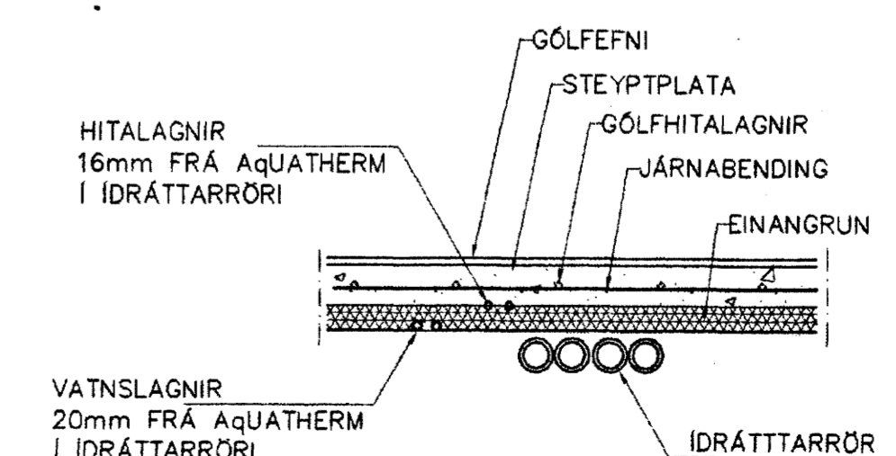
LAGNIR, SNID, 1:20
