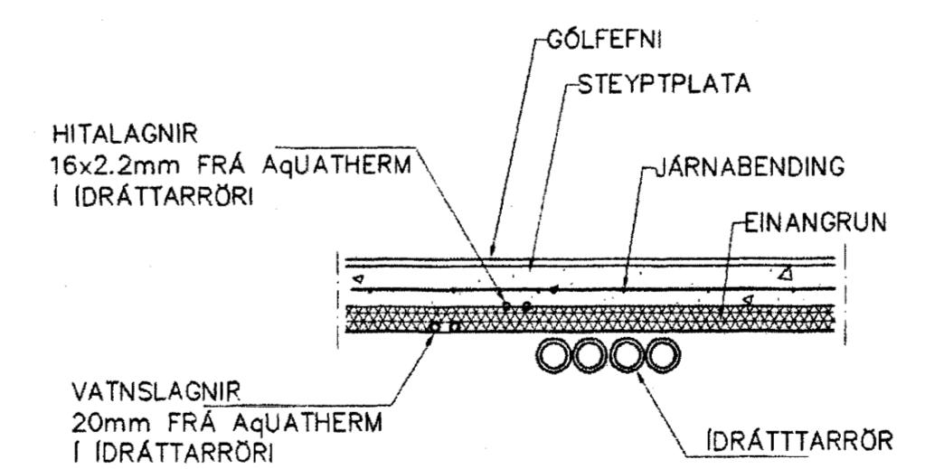
LAGNIR, SNID, 1:20
