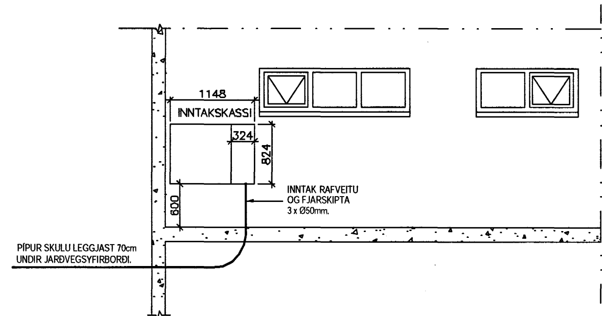
SNID C-C
