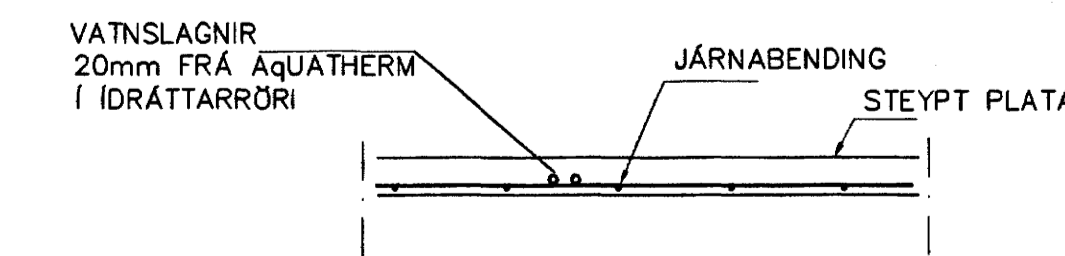
LAGNIR, SNID, 1:20
