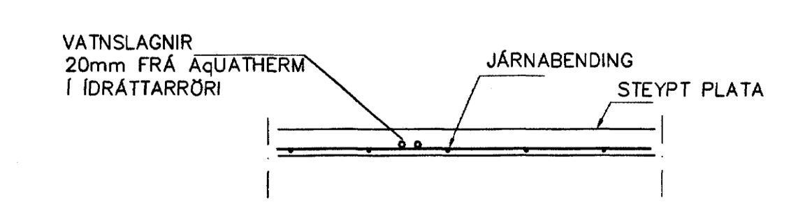
LAGNIR, SNID, 1:20
