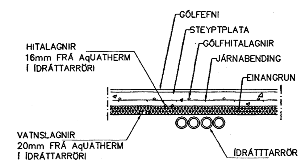
LAGNIR, SNID, 1:20
