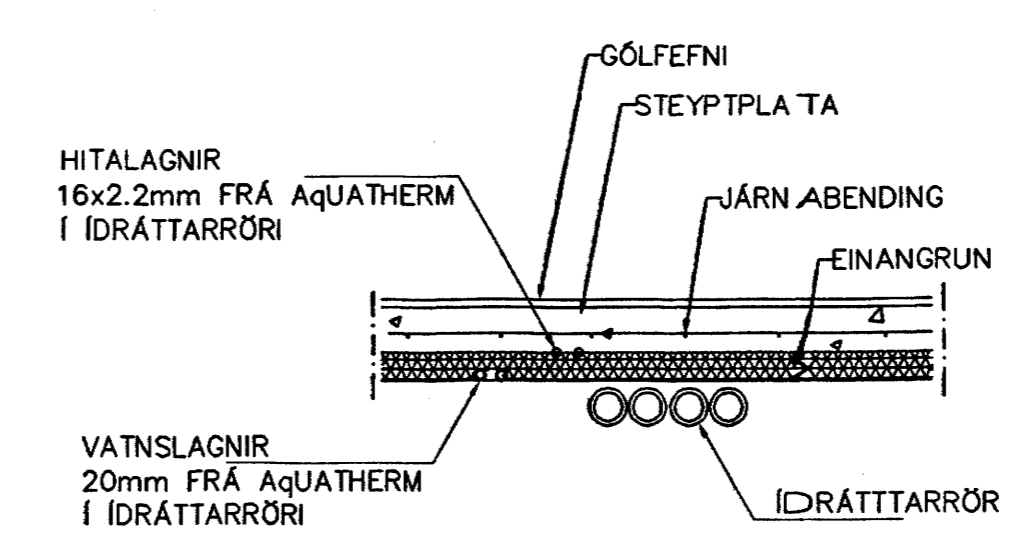
LAGNIR, SNID, 1:20
