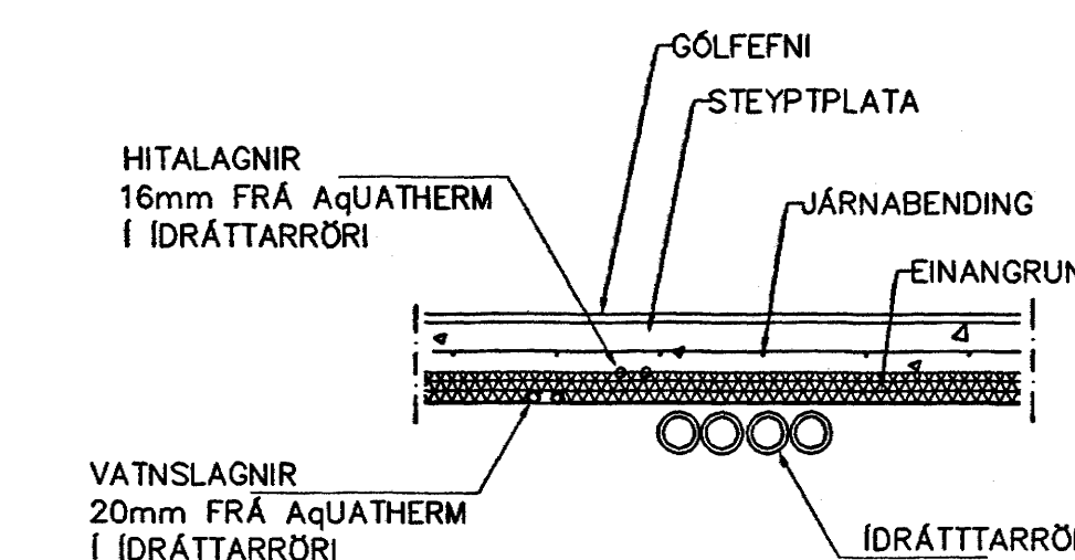
LAGNIR, SNID, 1:20
