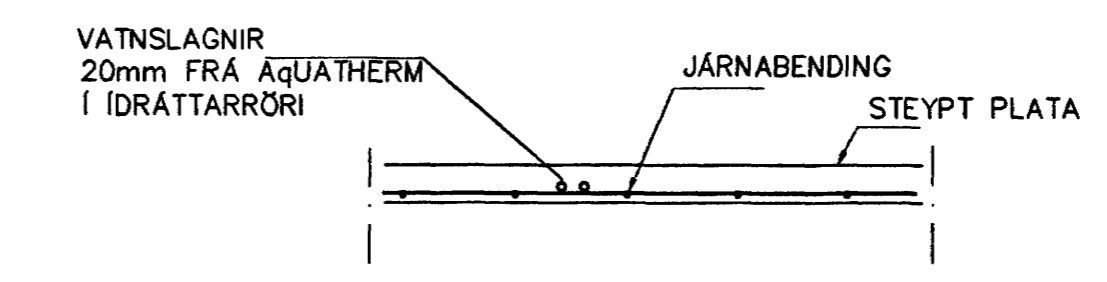
LAGNIR, SNID, 1:20
