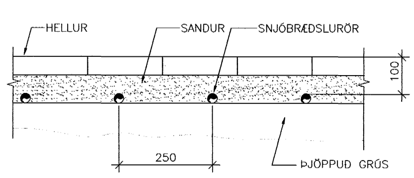
A SNID 1:10 HELLUR
