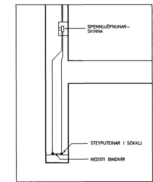
SNID TENGING SÖKKULSKAUTS
