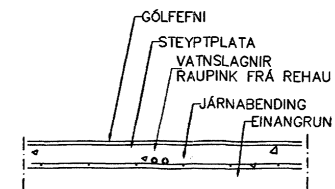
LAGNIR, SNID, 1:20
