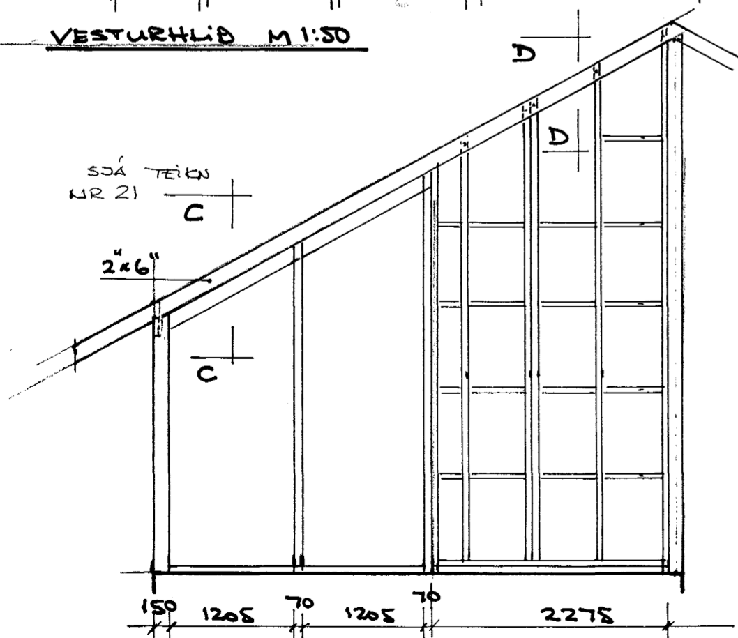
SUDURGAFL 1:50
