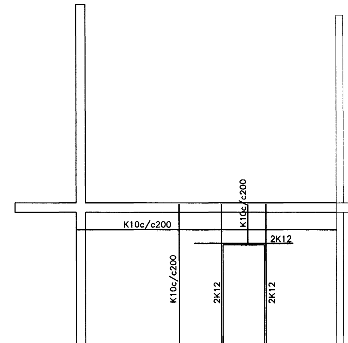
VEGGUR A 1:50
