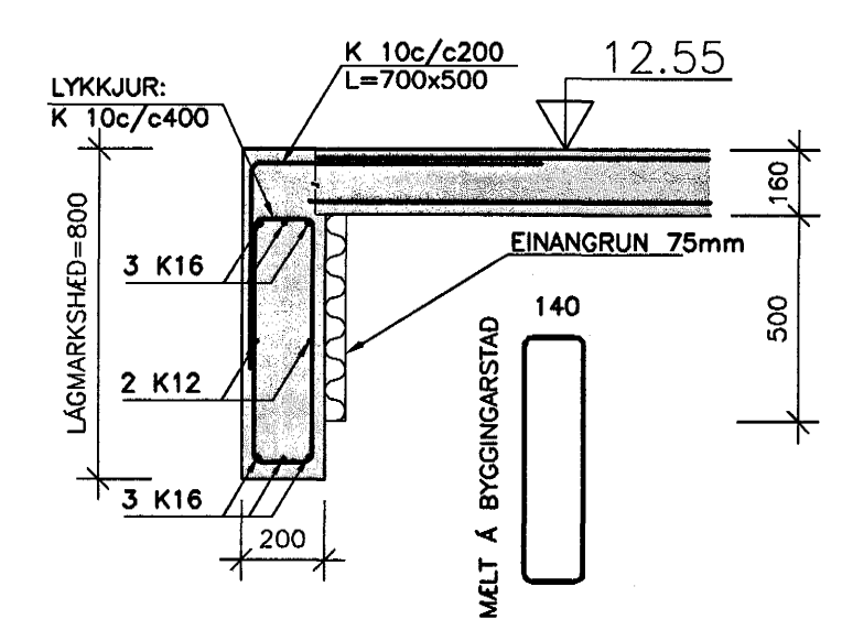
SNID B 1:20 B01 B02
