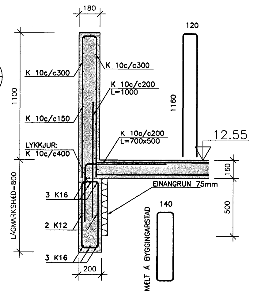
SNID A 1:20 B01 B02
