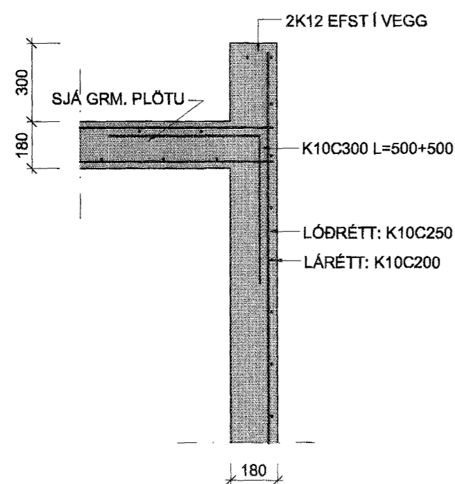
SNID C-C 1:20
