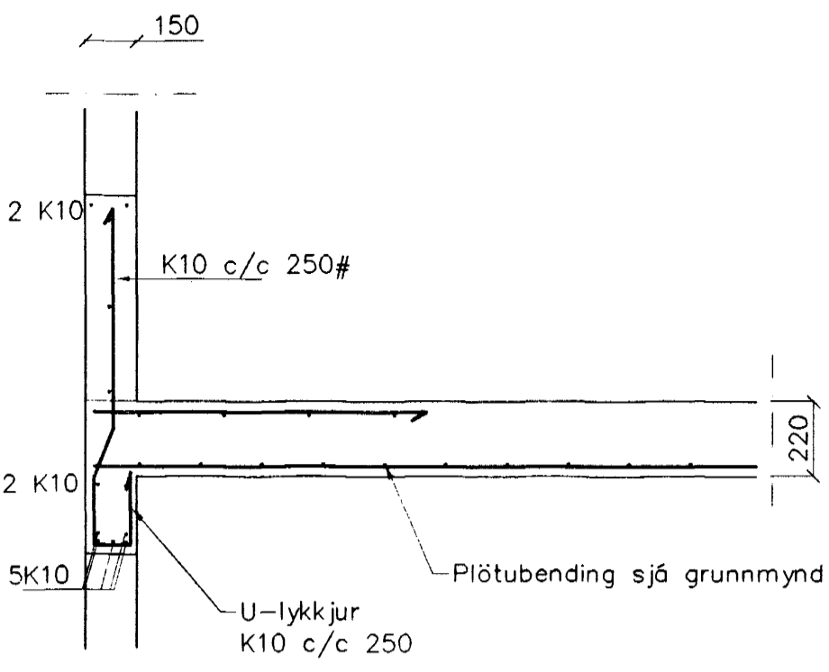
SNID 9 1:20
