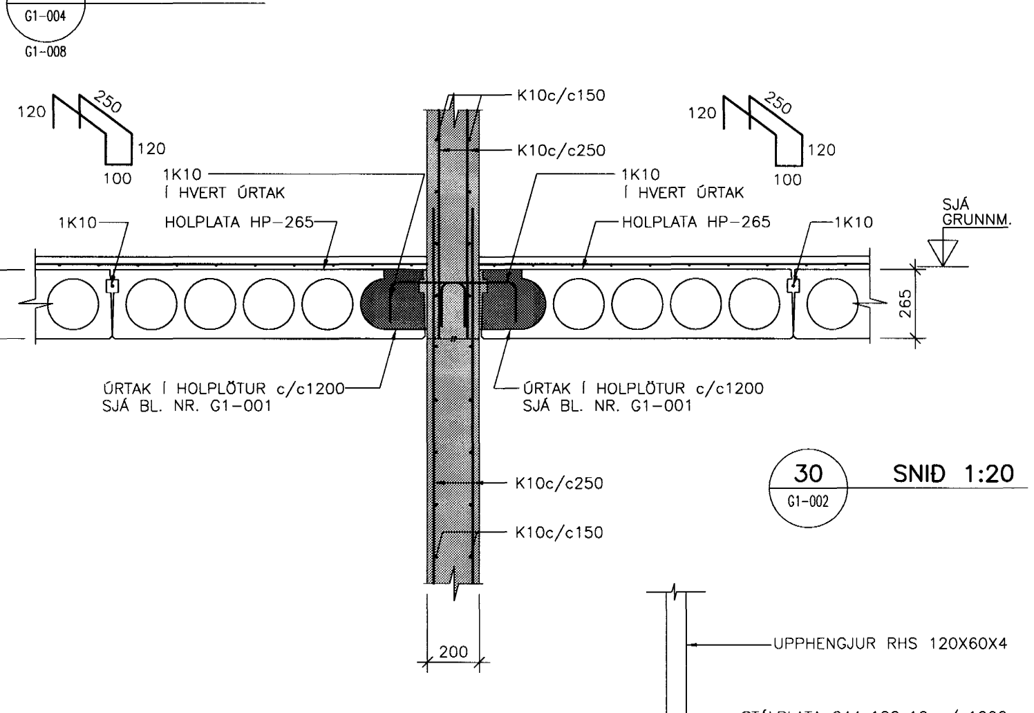
23 SNID 1:20
