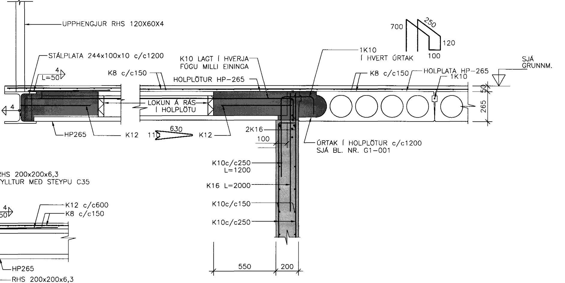
30 SNID 1:20
