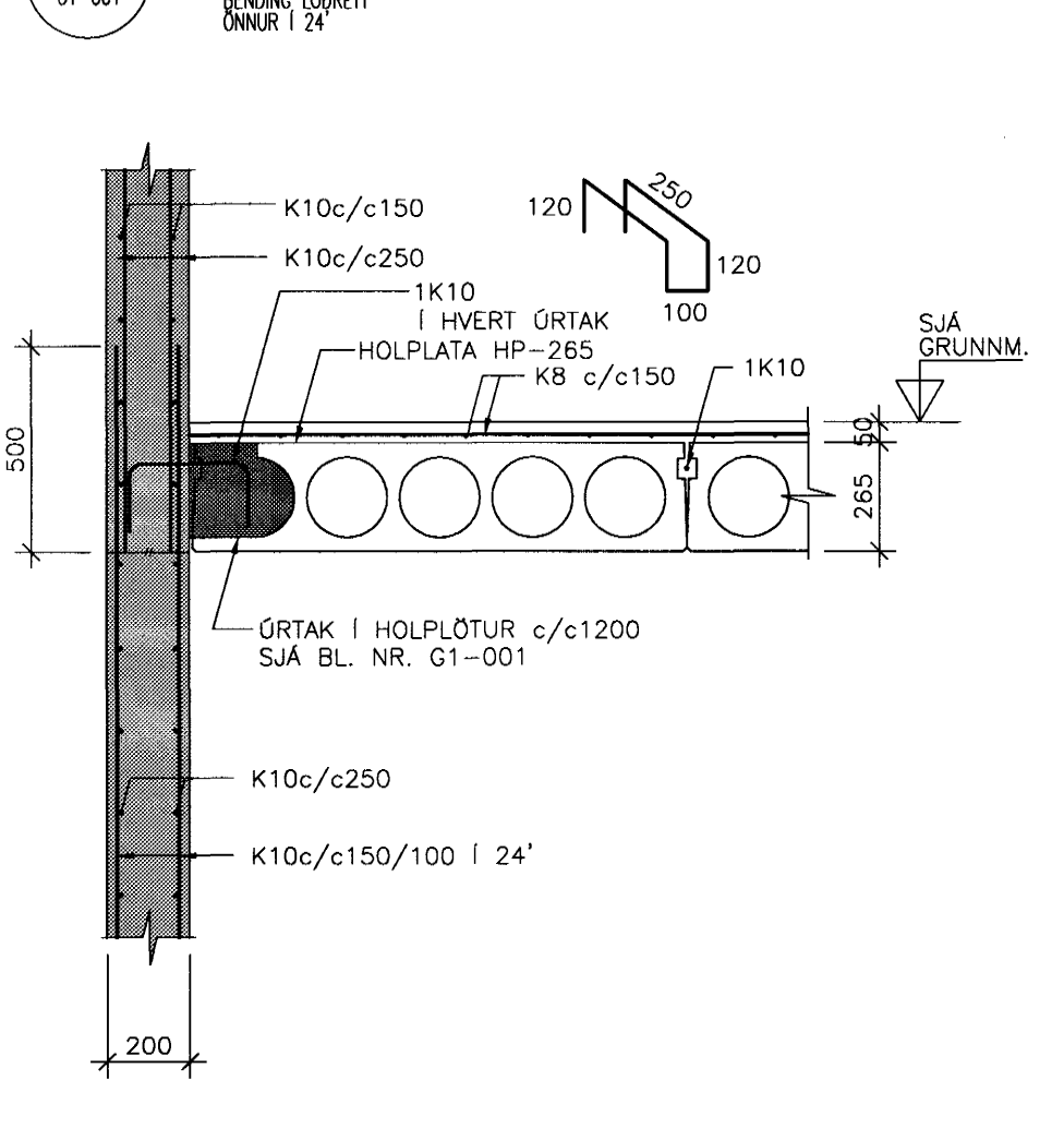
29 SNID 1:20
