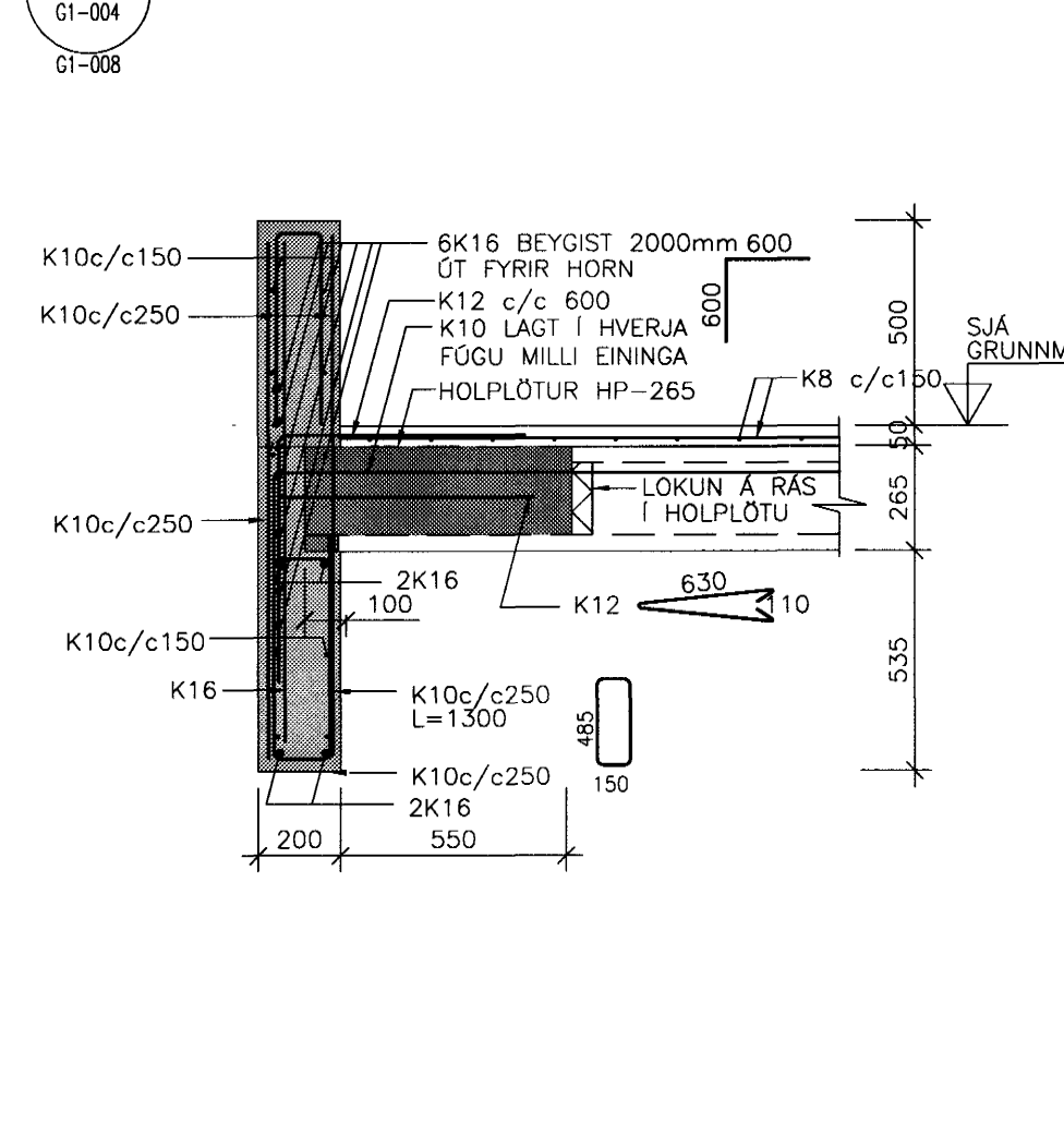
21 SNID 1:20
