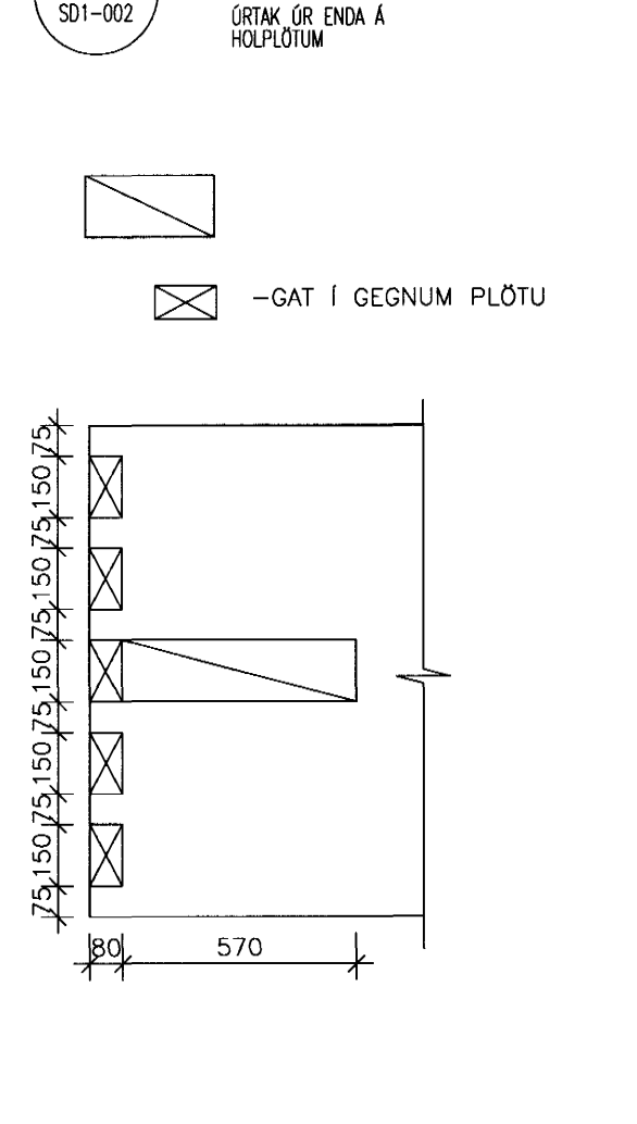
28 SNID 1:20
