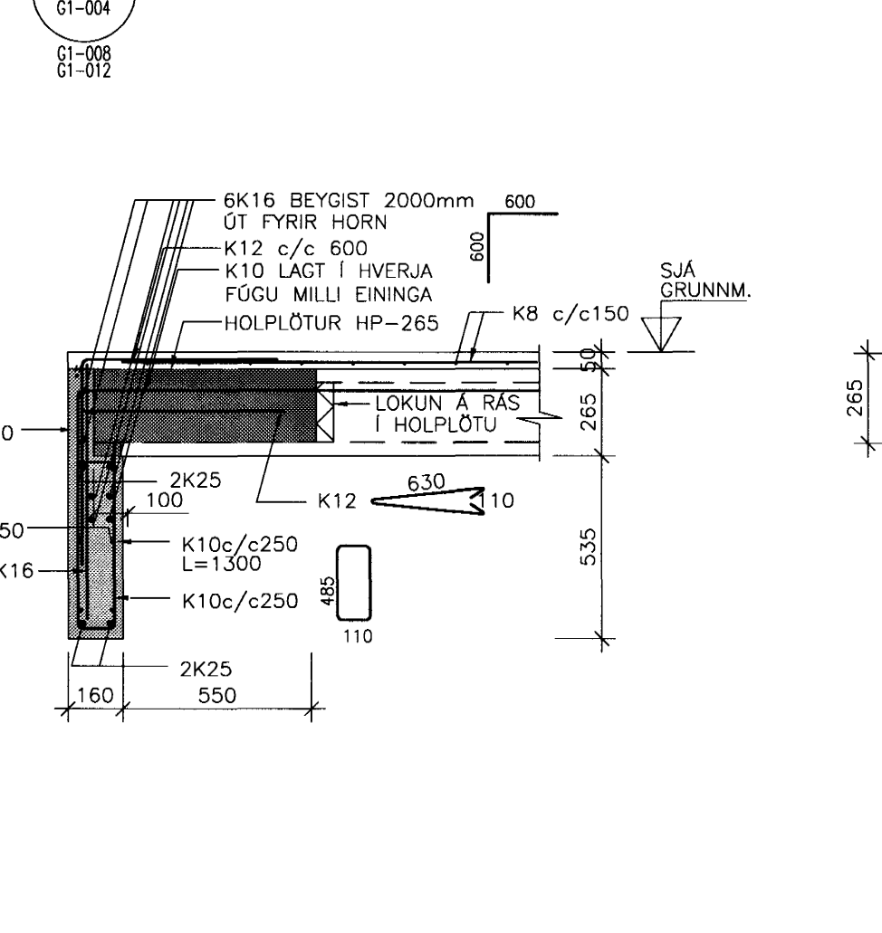
22 SNID 1:20
