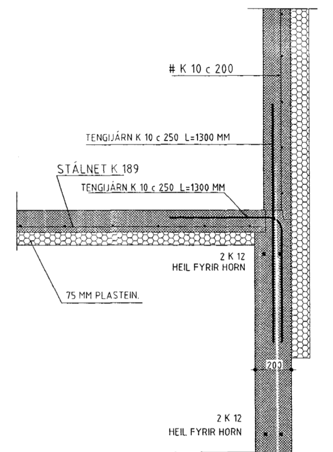
SNID - A 1:20
