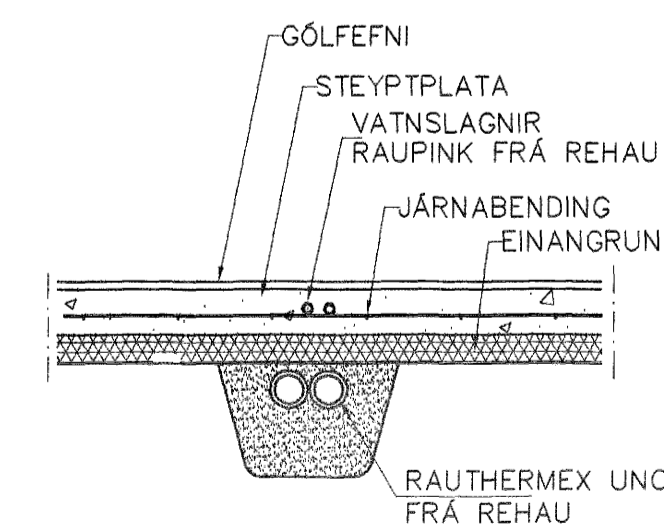
LAGNIR, SNID, 1:20
