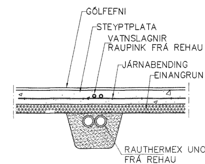
LAGNIR, SNID, 1:20
