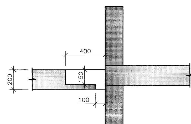
A SNID 1:20
