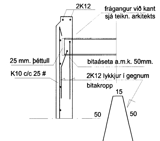
SNID C-C 1:20
