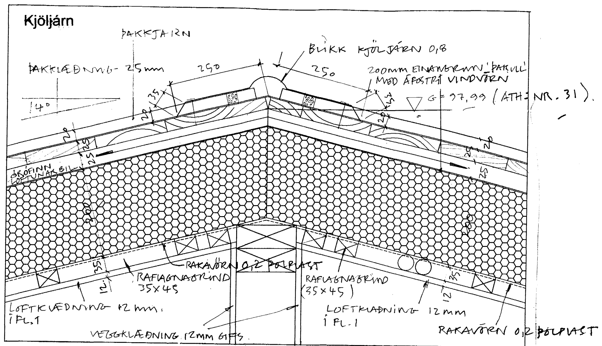
Sneiðing h-h mkv.1:5
