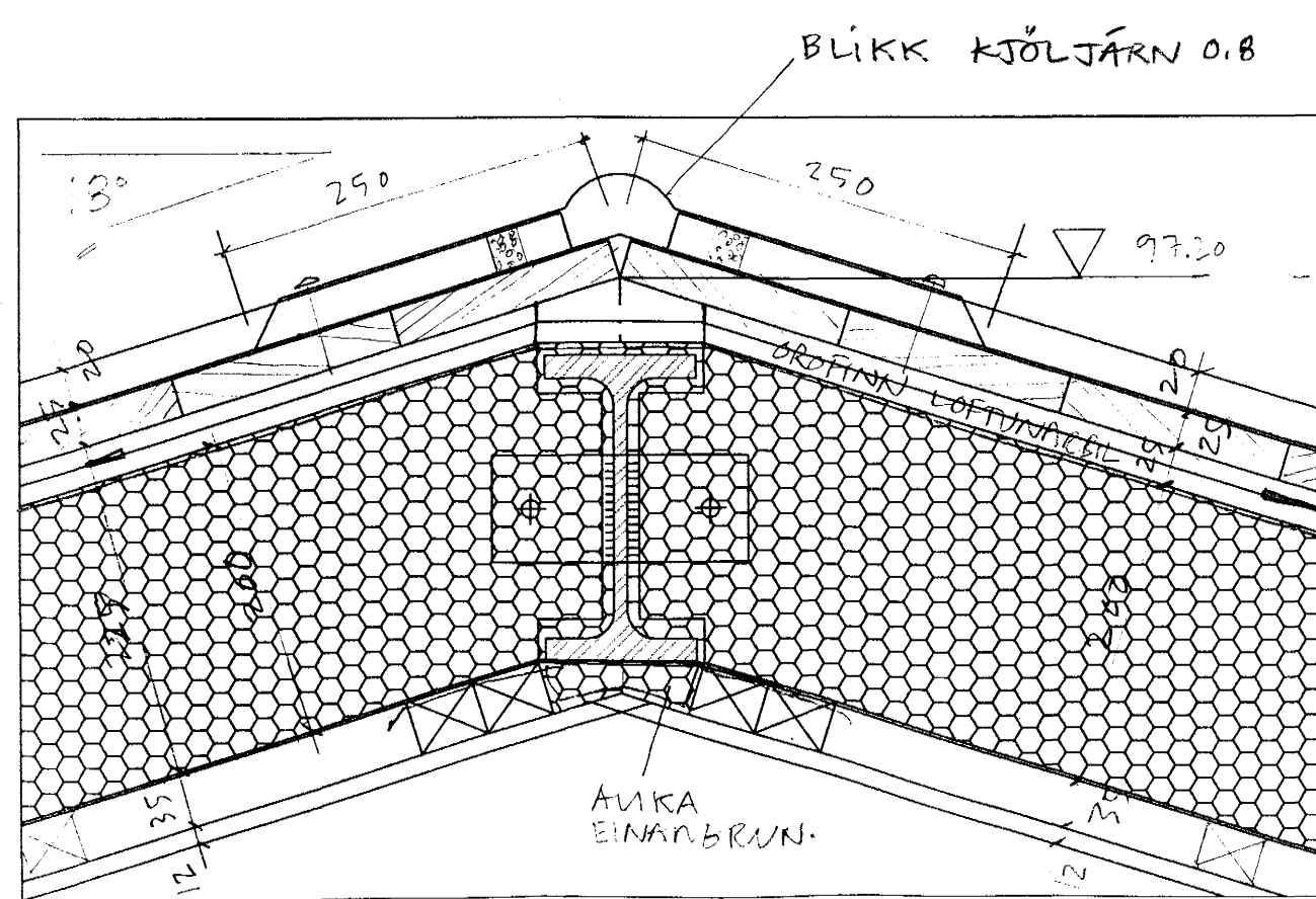
Sneiðing j-j mkv.1:5
