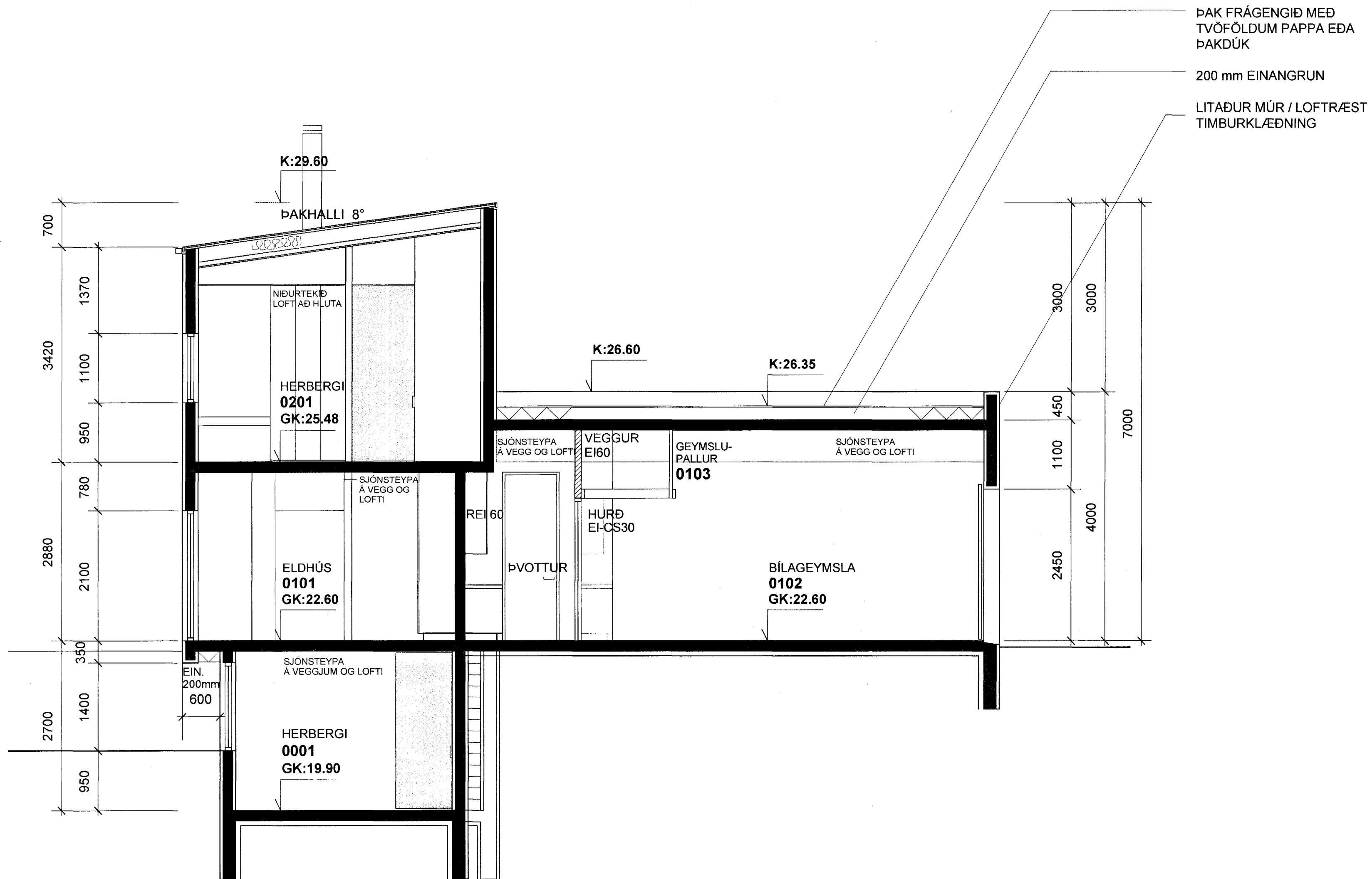
SNID B-B
