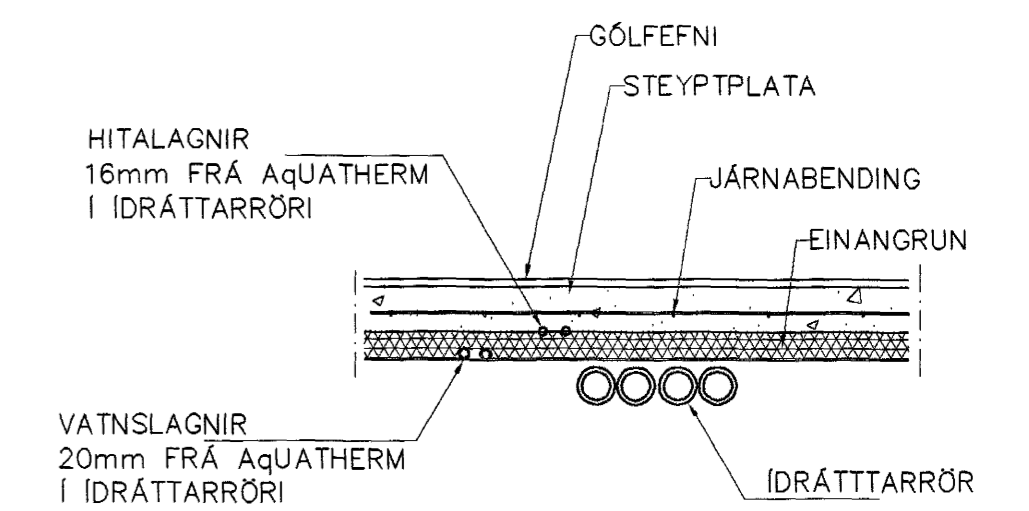
LAGNIR, SNID, 1: 20
