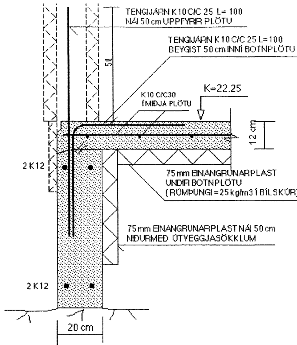
SNID E-E MKY. 1:10
