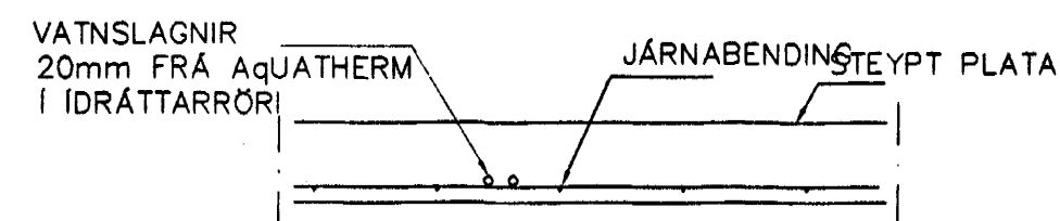
LAGNIR, SNID, 1:20
