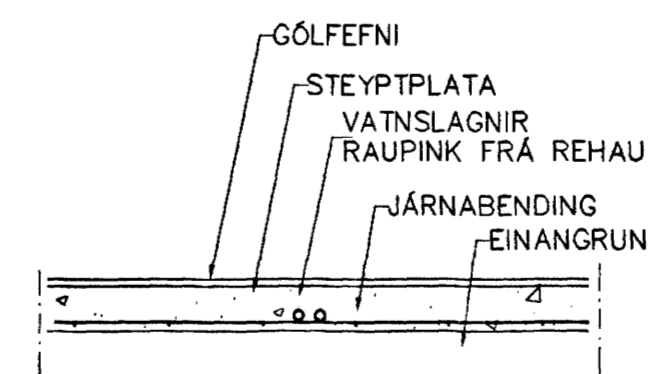
LAGNIR, SNID, 1:20
